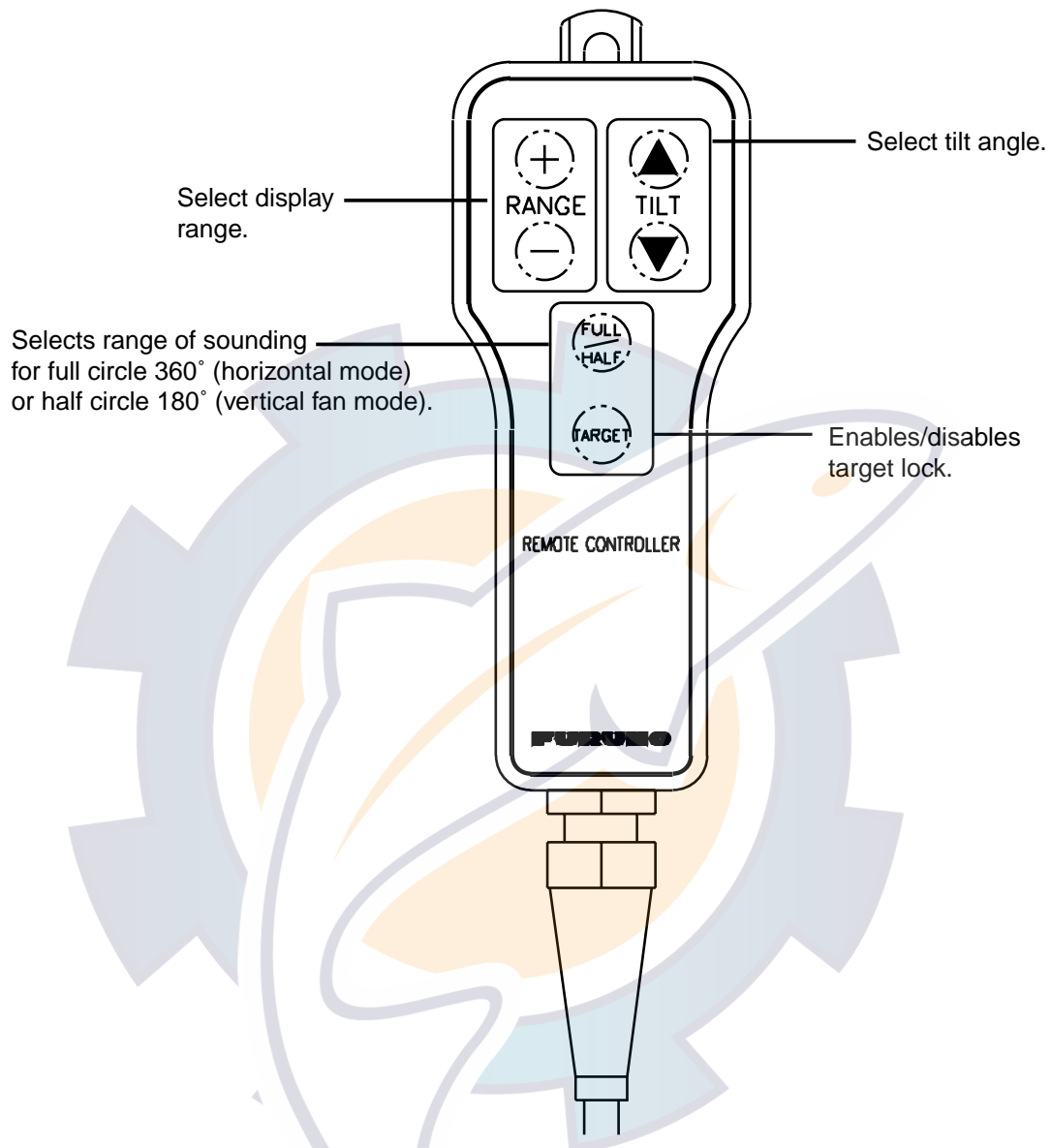
Figure 1-2 Remote controller
