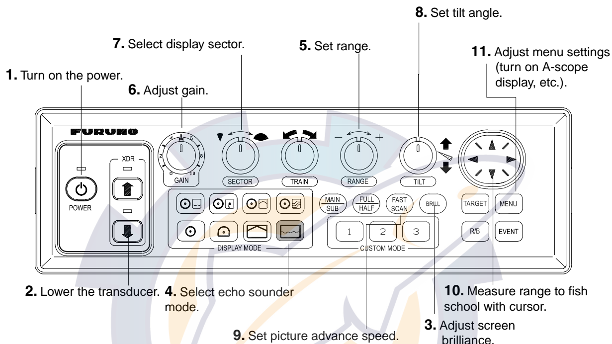
Figure 4-1 Control panel
