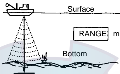
Figure 4-3 Range concept
