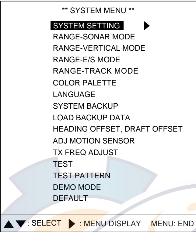
Figure 5-3 System menu
