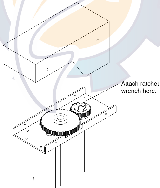
Figure 6-1 Hull unit
