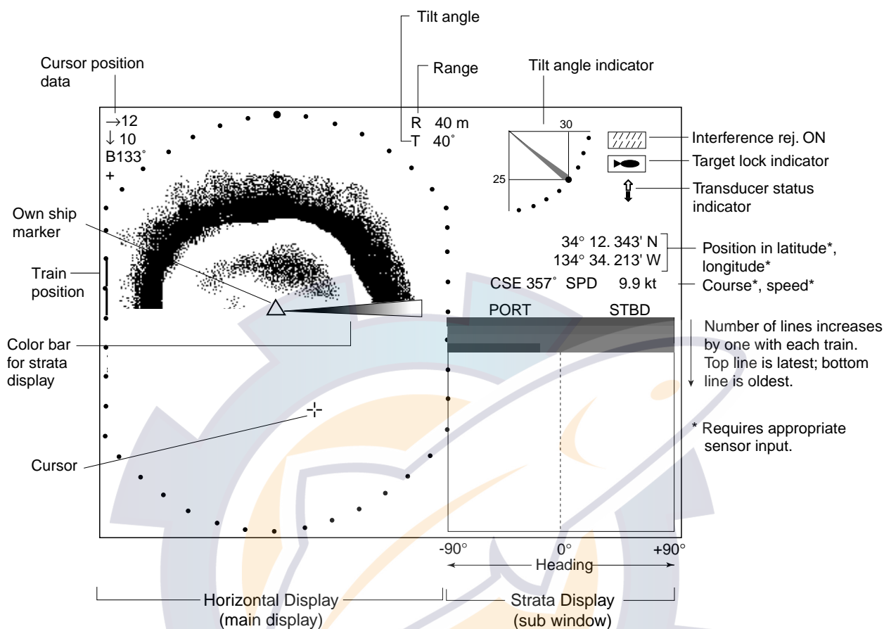
Figure 2-29 Horizontal/strata display
