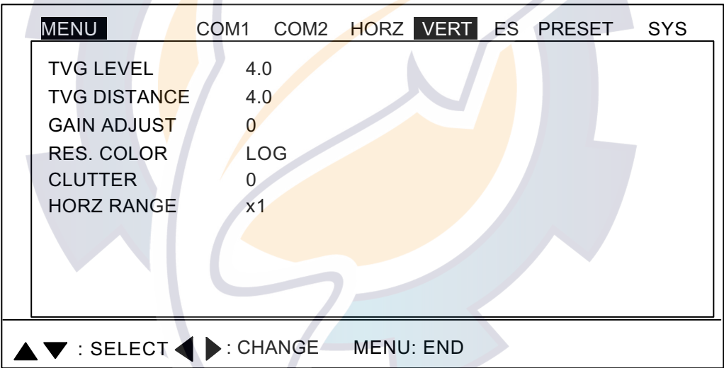
Figure 3-13 VERT menu
