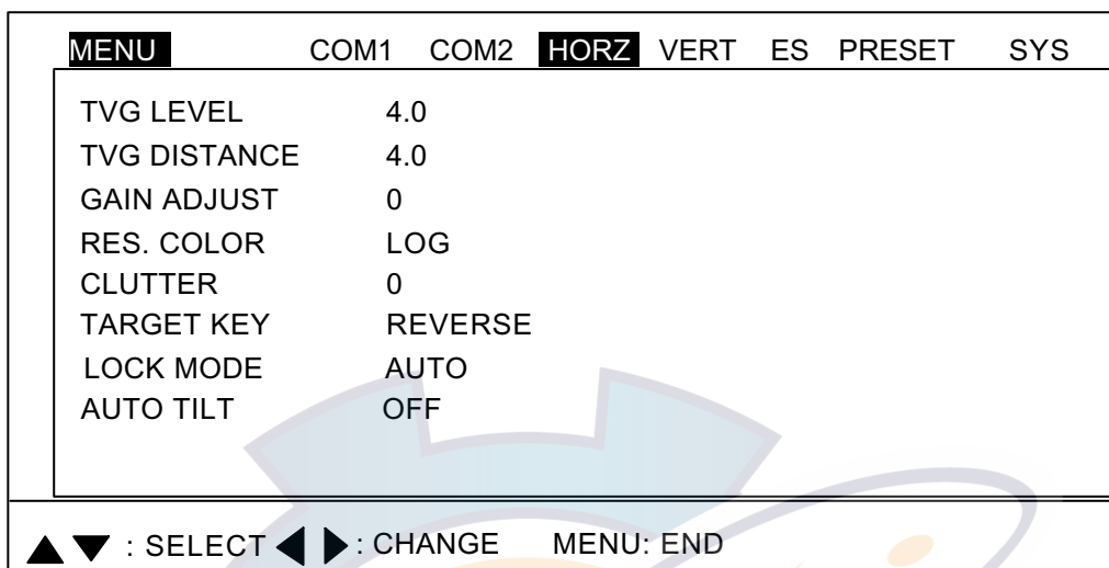
Figure 2-15 HORZ menu
