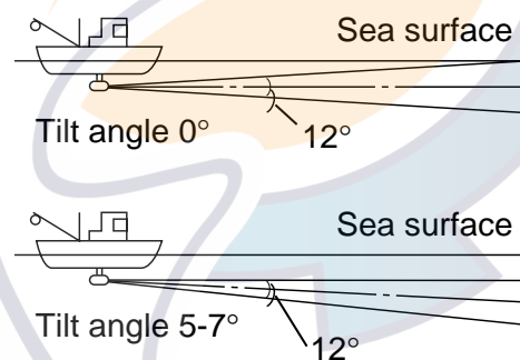
Figure 2-8 Tilt angle
