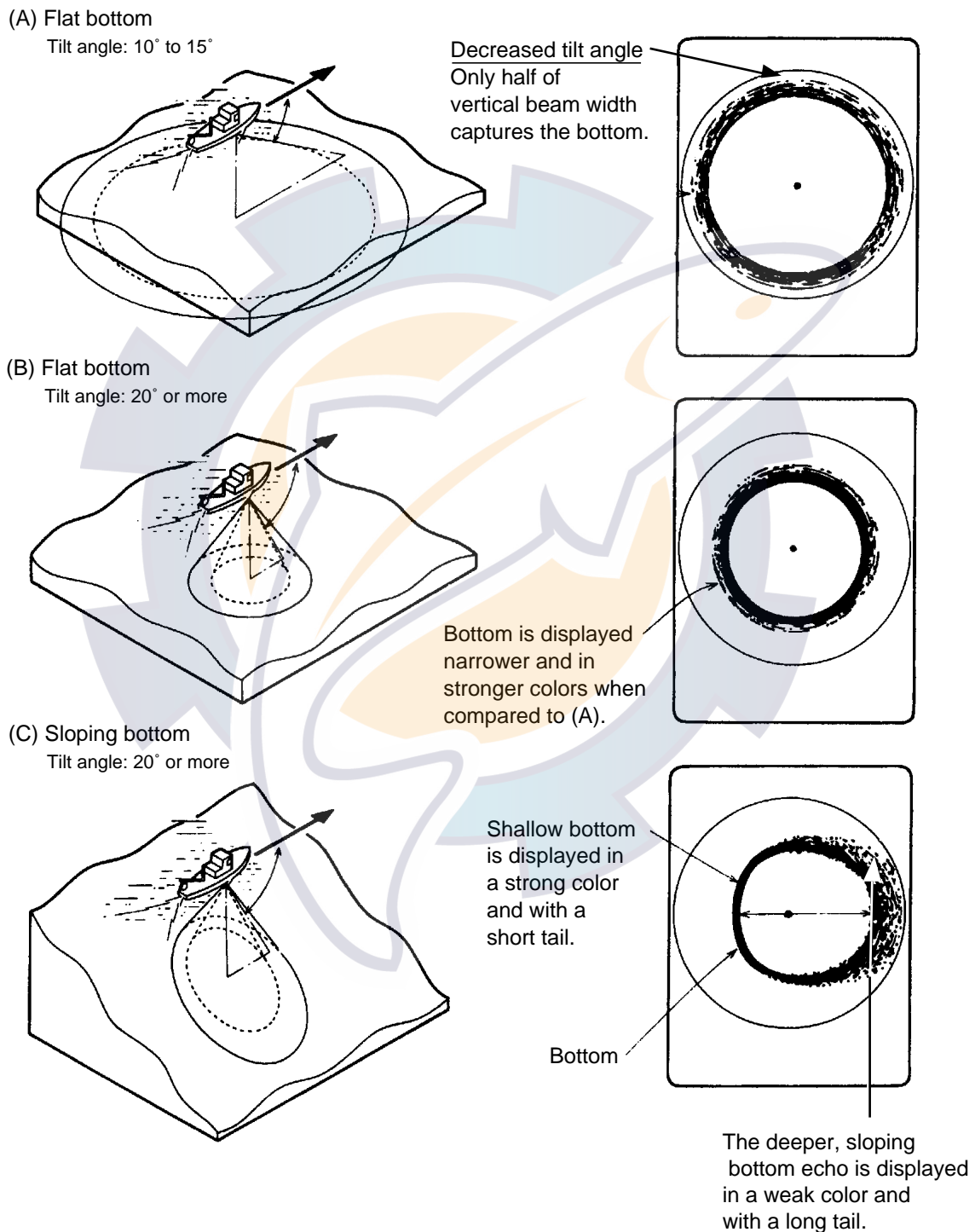
Figure 2-21 Bottom echoes
