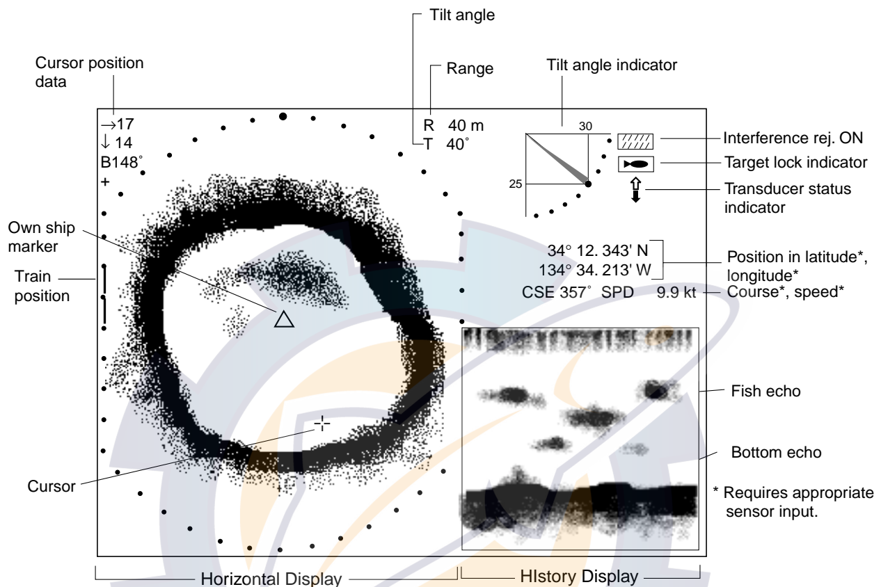
Figure 2-27 Horizontal/history display
