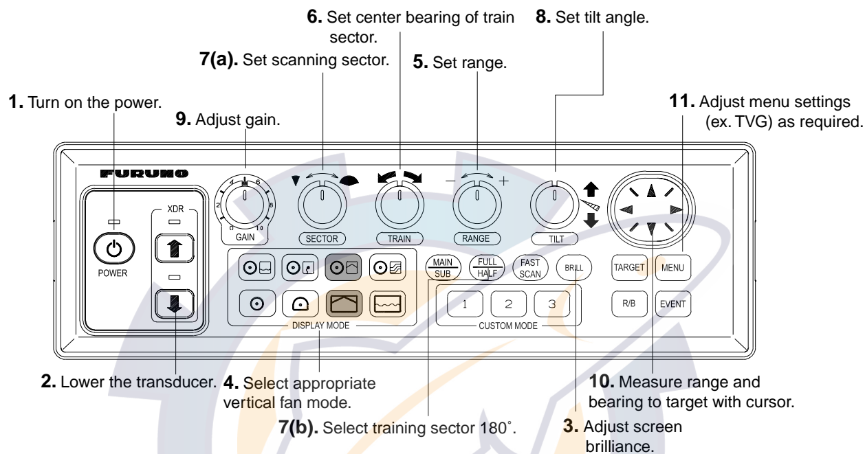
Figure 3-1 Control panel
