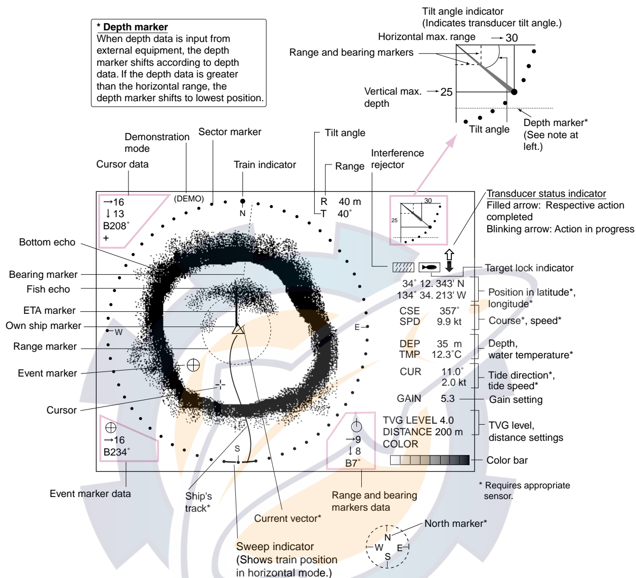
Figure 2-2 Typical horizontal mode display
